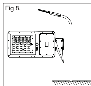
Fig 8. Adjust & balance, secure the fitting by tightening all four screws
