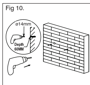
Fig 10. Drill 2 holes, ø14mm, depth 60mm, 104mm apart.
