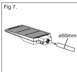
Fig 7. Screw fitting onto the pole (size ø50mm).
